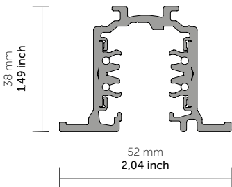
A9000R: Recessed
