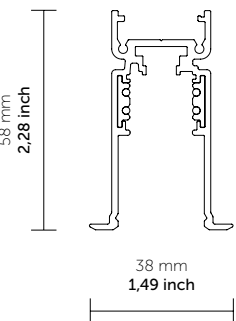
ST18: Recessed
