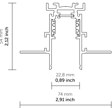
ST5: Recessed
