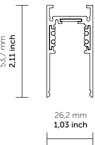
ST2: Suspended
