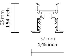
ST8: Recessed
