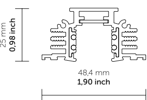
ST3: Recessed
