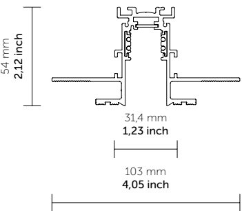
ST10: Recessed
