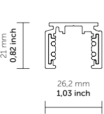
ST1: Surface
