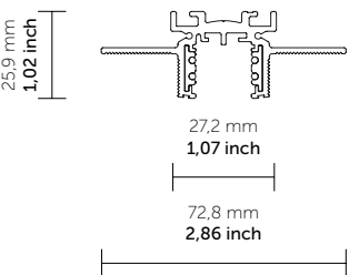
ST13: Recessed
