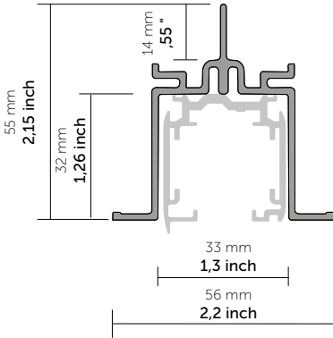
FTP: recessed
